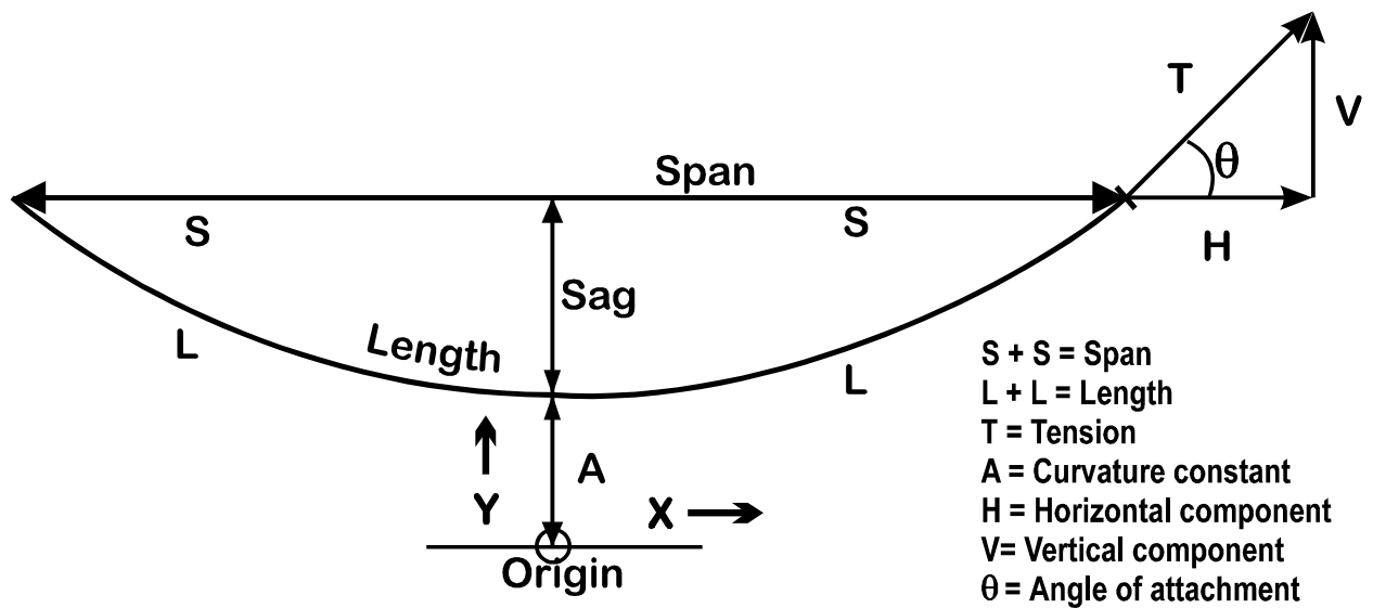
Figure 2 A level symmetrical treadway with its various parts labeled.
